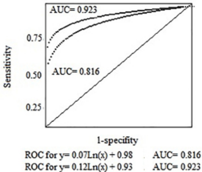
Figure 1. ROC values for the C-SSRS subscales
